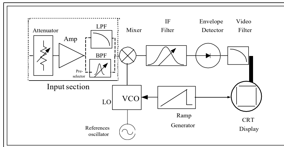
Figure 1. Simplified block diagram of Heterodyne spectrum analyzer
